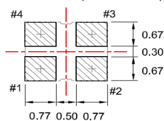
Land Pattern(REFERENCE)
