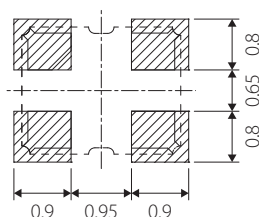
Land Pattern(REFERENCE)
